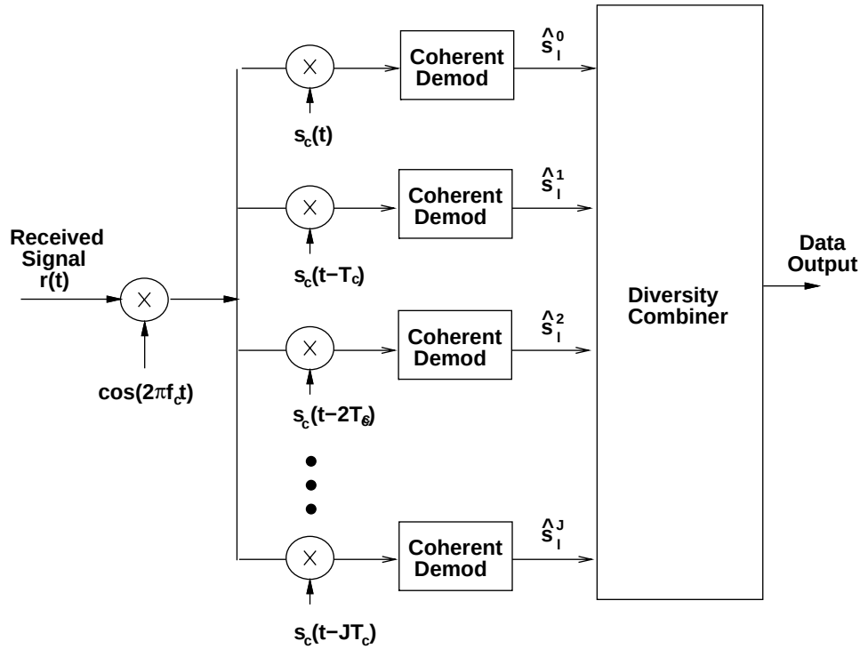
Figure 13.10: RAKE receiver
