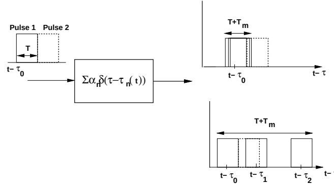
Figure 3.11: Multipath Resolution.
