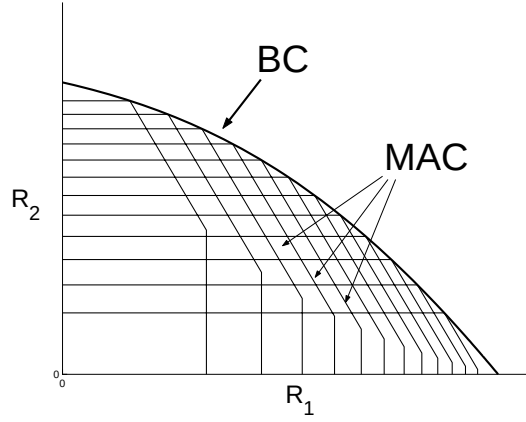
Figure 14.15: AWGN Downlink (BC) Capacity Region as a Union of Capacity Regions for the Dual Uplink (MAC)
