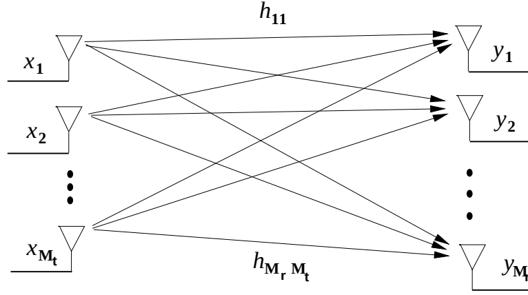
Figure 10.1: MIMO Systems.
