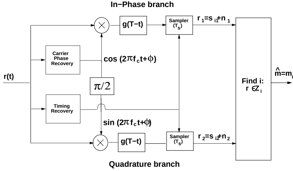
Figure 5.28: Receiver Structure with Carrier and Timing Recovery.
